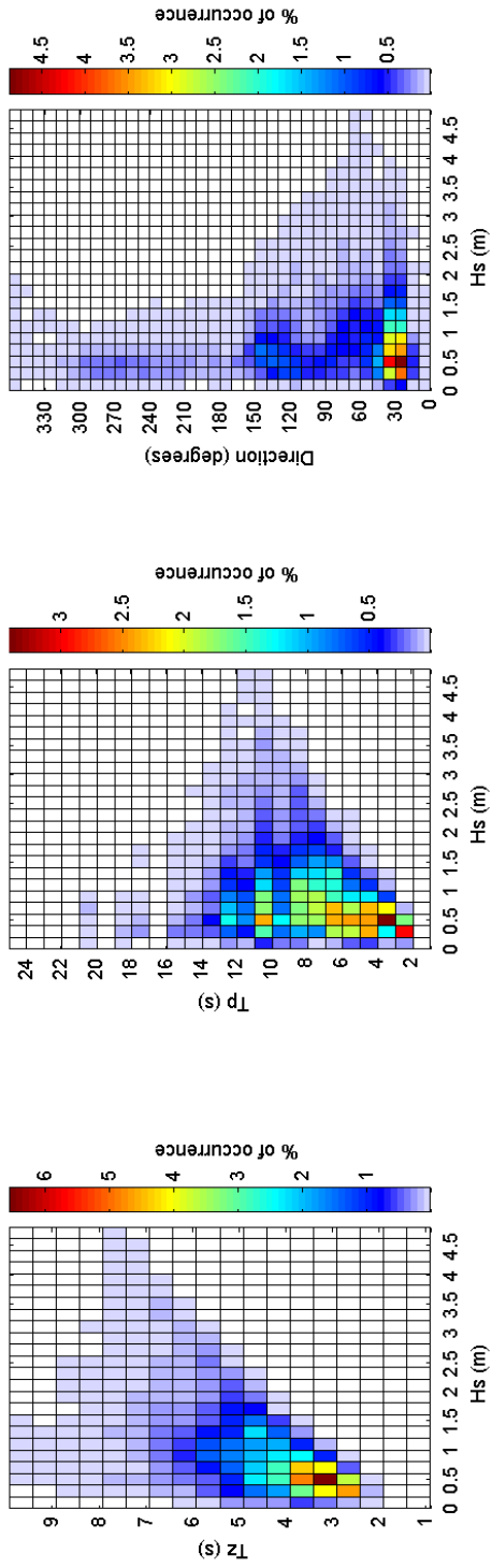
Hornsea 2008 to 2010 - Joint distribution (% of occurrence)
